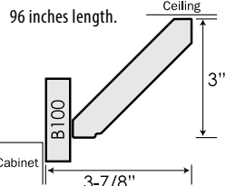
A140 ANGLED CROWN MOULDING
