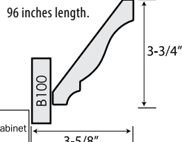
A141 ANGLED CROWN MOULDING
